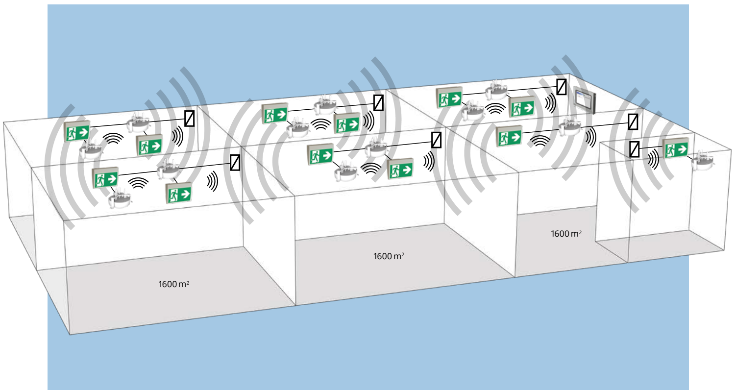
Example of an industrial hall with virtual fire zones
