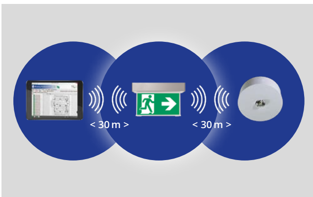
Wireless luminaire monitoring and control with Wireless Professional (left) and Wireless Basic® (right)
